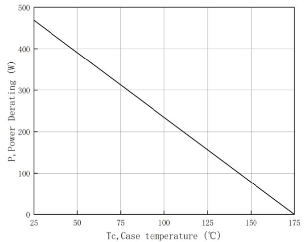
Figure 4. Power Derating
