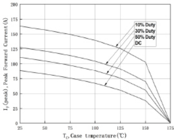
Figure 3. Current Derating
